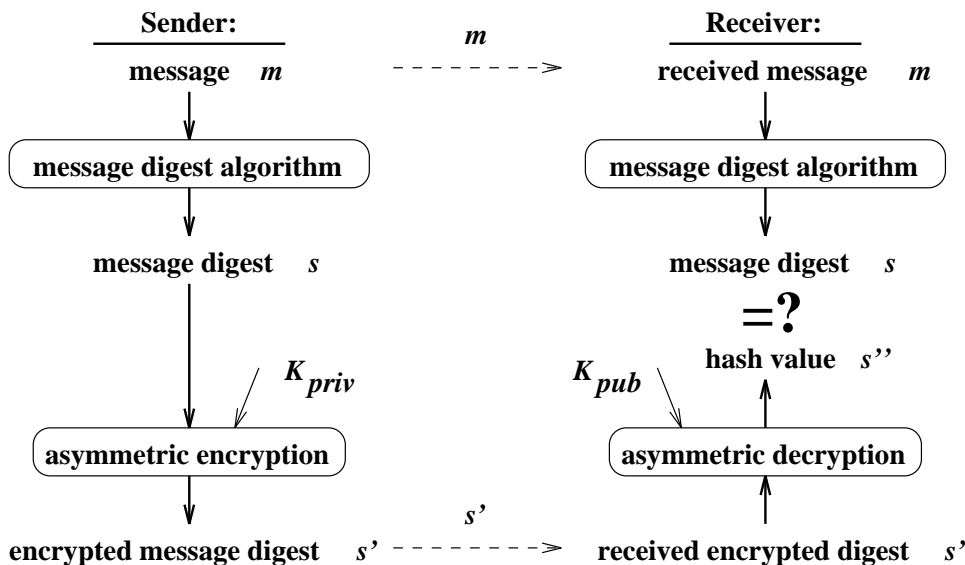
Figure 2: Digital signature generation and validation
